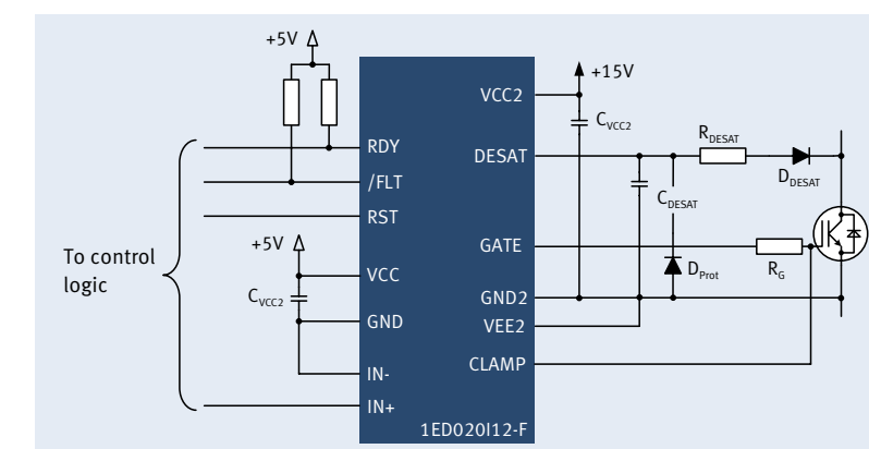
Typical application 1ED020I12-F
