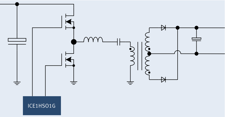
LLC Resonant (No SR)
