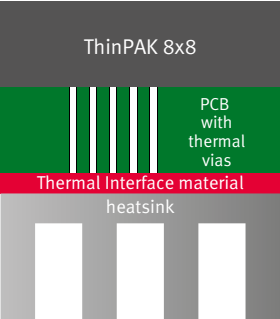
Thermal cooling system for ThinPAK 8x8
