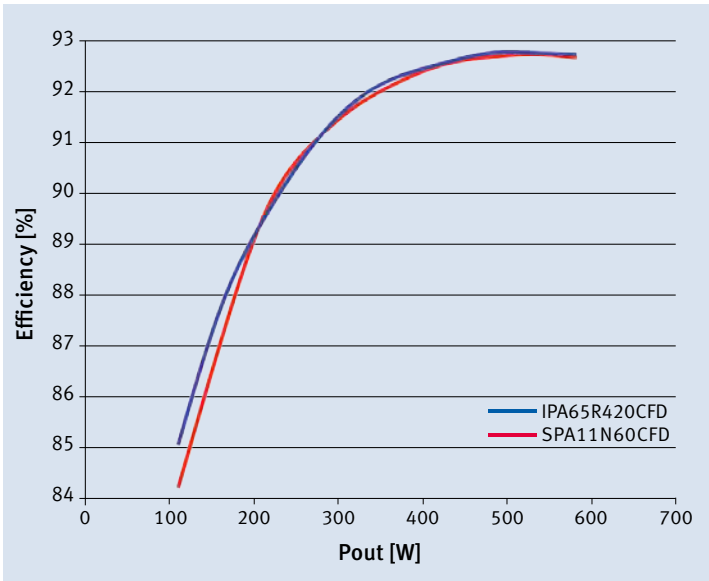
CFD vs. CFD2 efficiency comparison in a 12 V Server SMPS used Topologie ZVS FB @ 100 kHz
