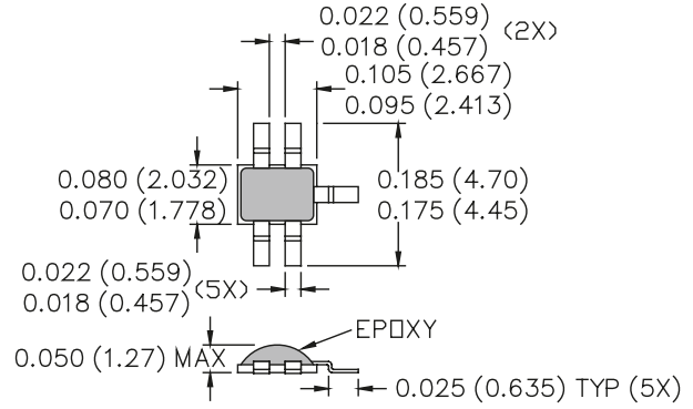
E50SM
